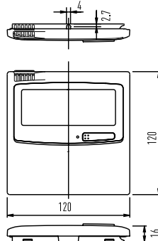
WIRELESS REMOTE CONTROLLER (CZ-RWSU2, CZ-RWSC2)
