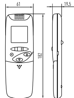
WIRELESS REMOTE CONTROLLER (CZ-RWSU2, CZ-RWSC2)
